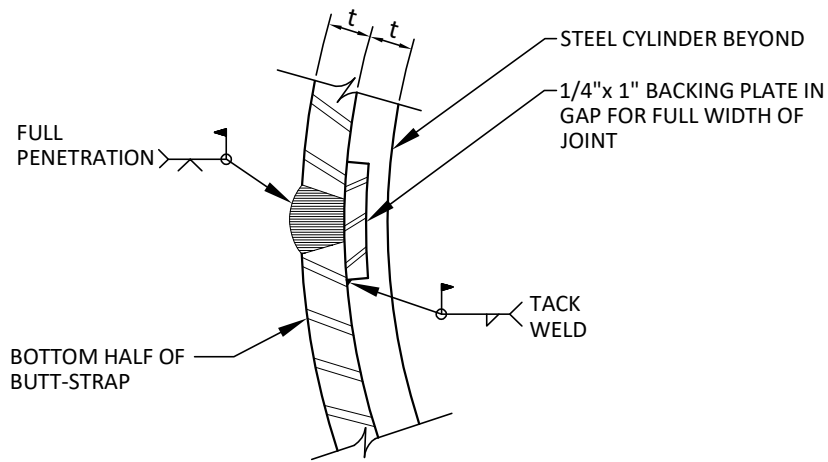
BUTT-STRAP SPLICE
