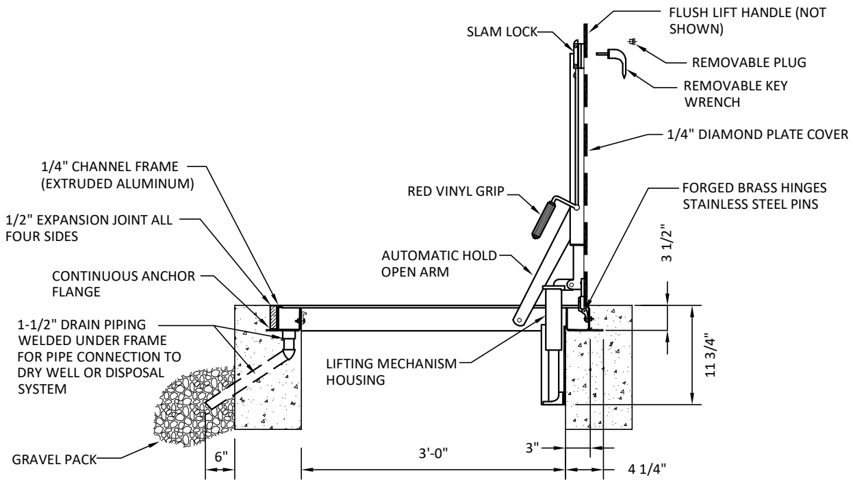
SECTION A
