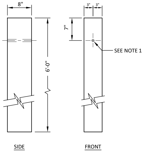
6" x 8" WOOD POST SEE NOTE 3
