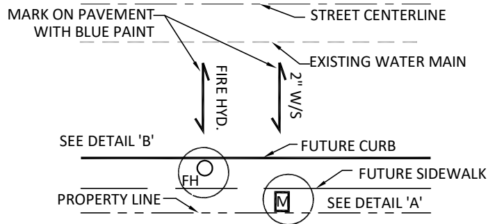
SERVICE LOCATION PLAN
