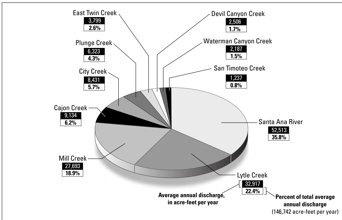
Figure 12. Average annual discharge of gaged streams flowing into the San Bernardino area, California, 1945–98.
