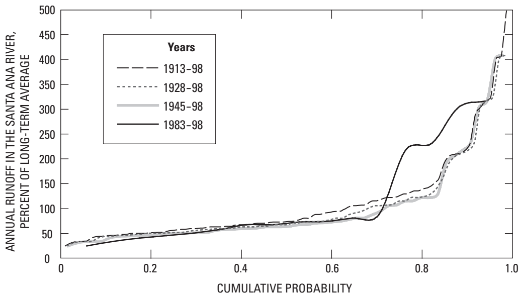
Figure 53. Cumulative probability of annual runoff in the Santa Ana River, San Bernardino area, California, for selected time periods, 1913–98. Calendar-year data for USGS gaging station 11051501.
