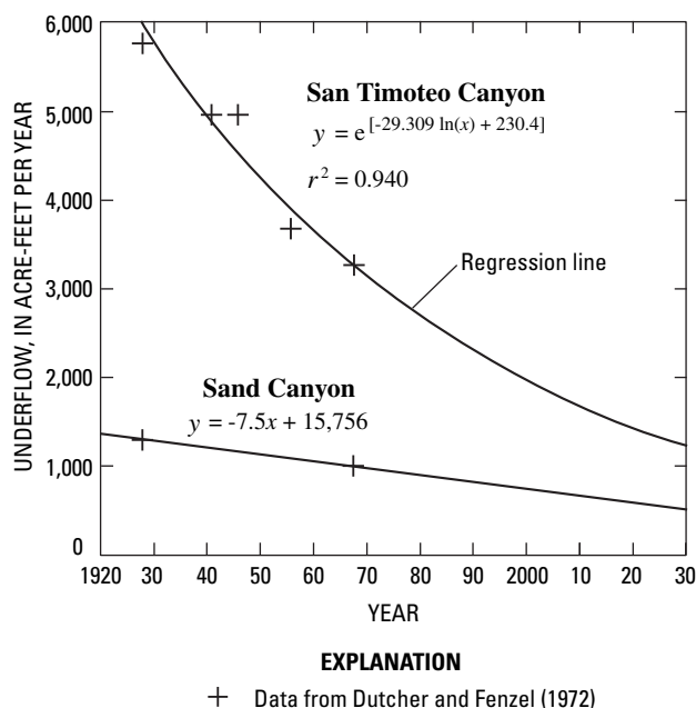
Figure 27. Estimated underflow from San Timoteo Canyon and Sand Canyon into the San Bernardino area, California.
