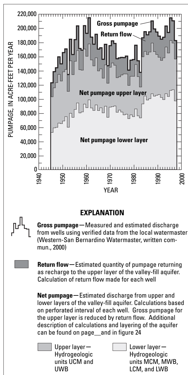
Figure 25. Annual ground-water pumpage for the San Bernardino area, California, 1945–98.
