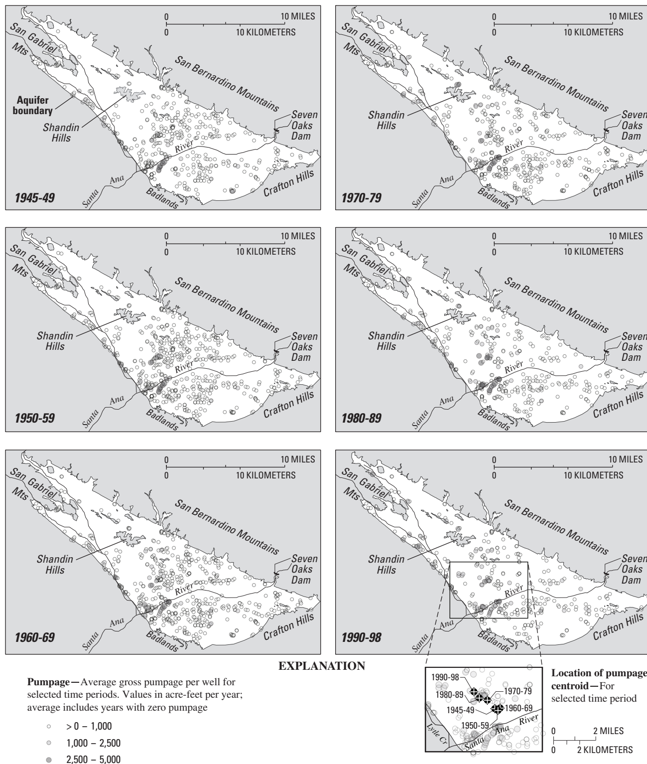
Figure 31. Areal distribution of average pumpage in the San Bernardino area, 1945–98.
