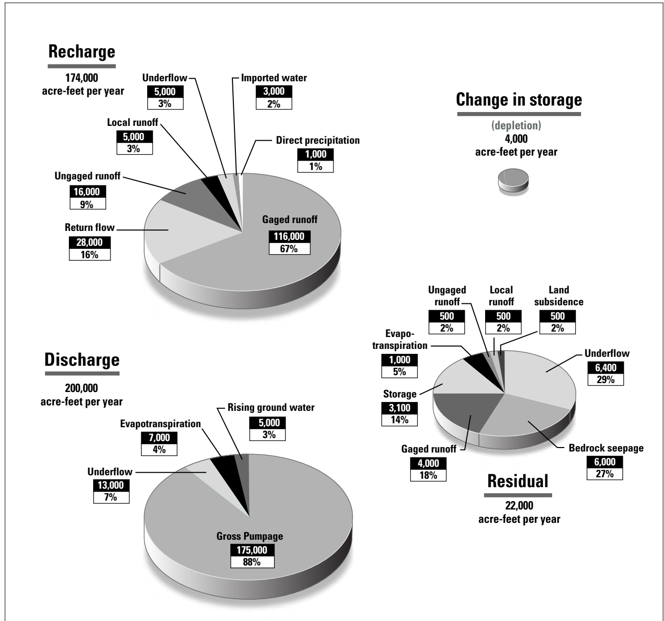
Figure 33. Average recharge, discharge, and change in storage for the valley-fill aquifer in the San Bernardino area, California, 1945–98. Values in acre-feet per year; individual components also shown as approximate percent of total recharge or discharge. Annual values listed in table 8. Residual represents difference between recharge, discharge, and change in storage; components of the residual are rough estimates.
