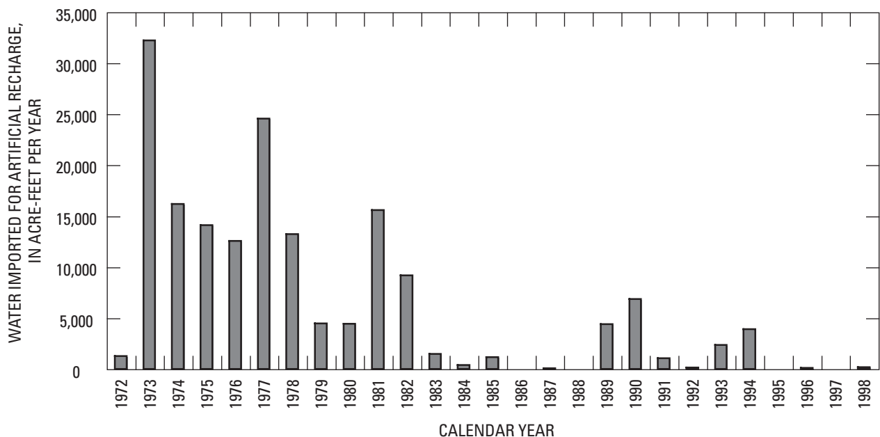
Figure 19. Water imported for artificial recharge into the San Bernardino area, California, 1972–98.
