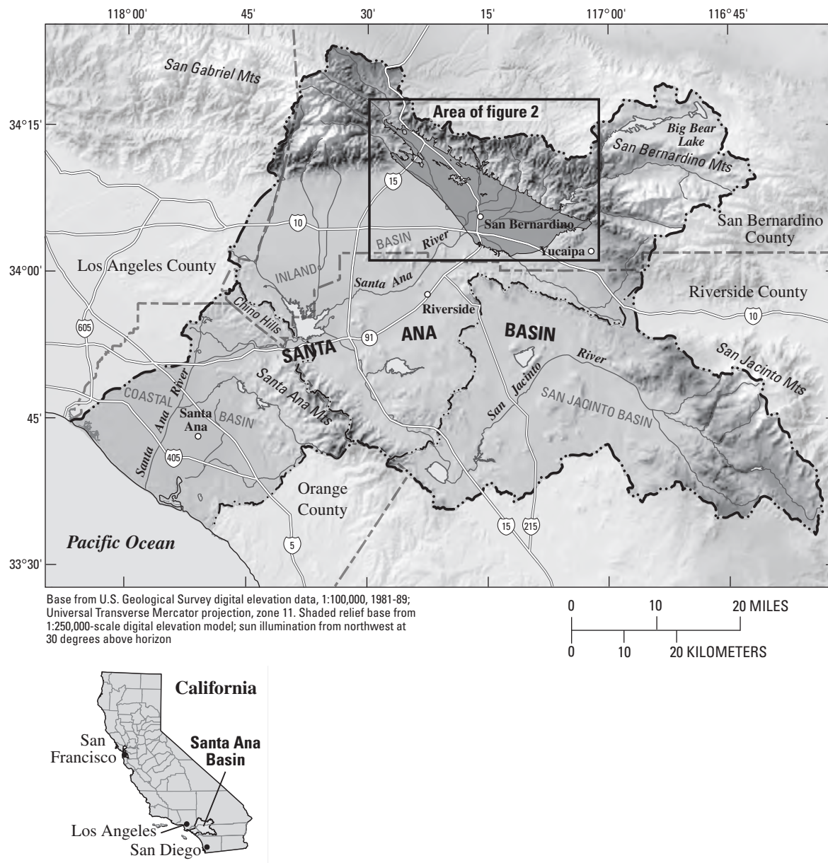
Figure 1. Location of the San Bernardino area in the Santa Ana River drainage basin, southern California.
