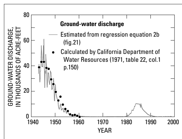
Figure 30. Ground-water discharge into Warm Creek in the San Bernardino area California, 1943–98.
