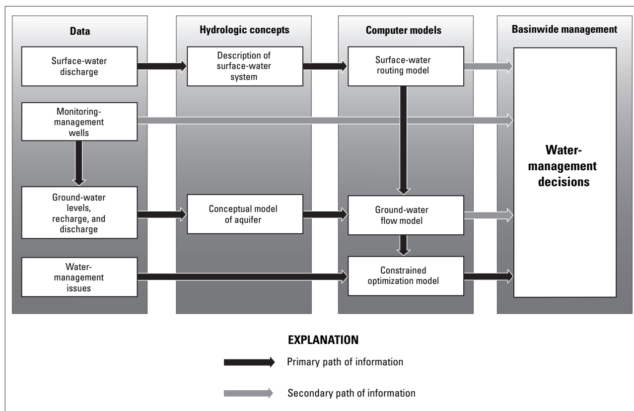
Figure 3. Major components and flow of information in this study of the San Bernardino area, California.
