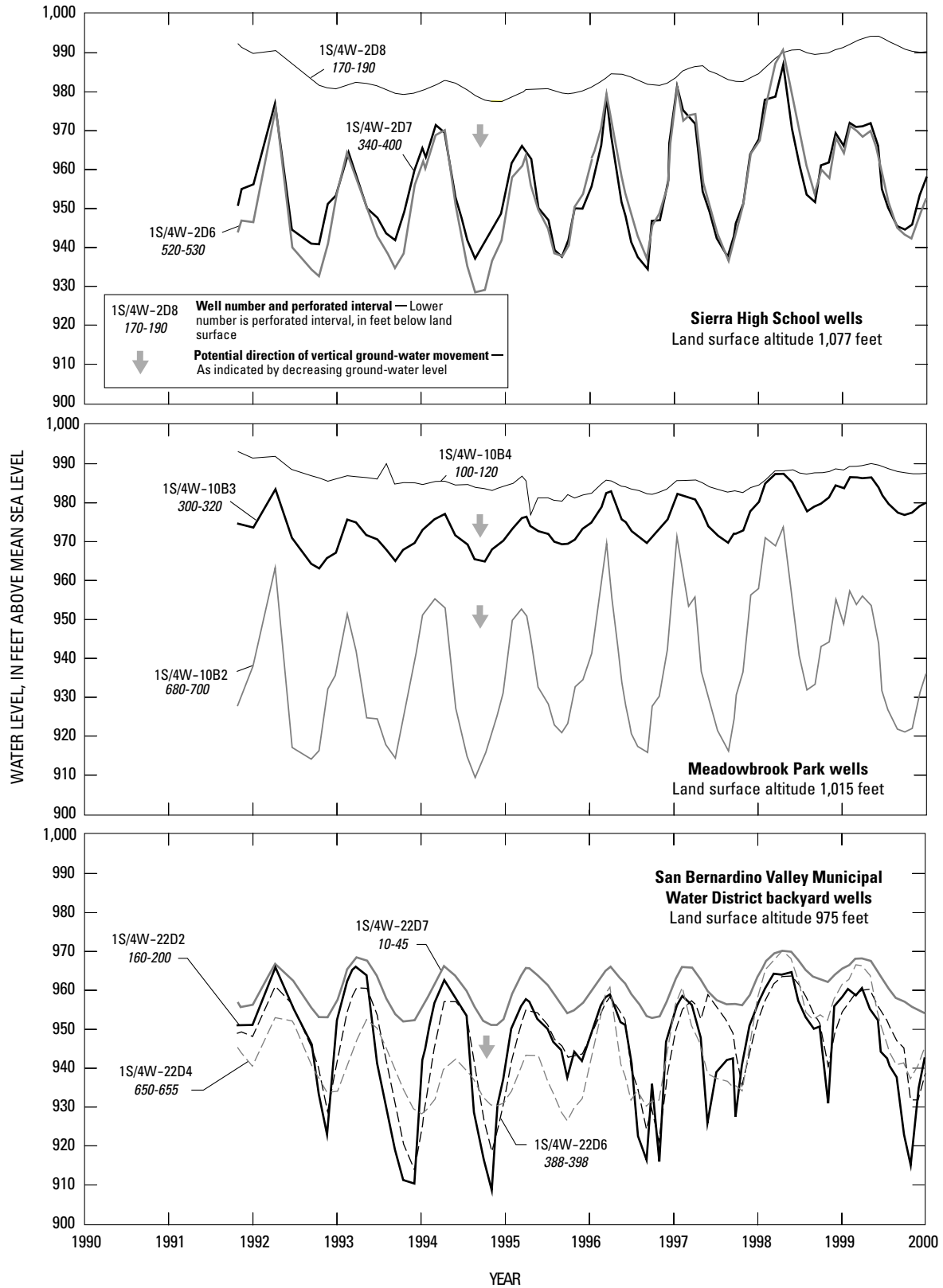
Figure 35. Measured water level in multiple-depth cluster wells in the San Bernardino area, California, 1990–2000.
