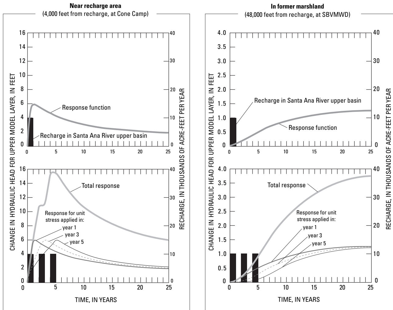
Figure 50. Superposition of response functions. Note different scale of graphs. Location of recharge (Santa Ana River upper basin) and water-level response (Cone Camp and SBVMWD) shown in figure 49.
