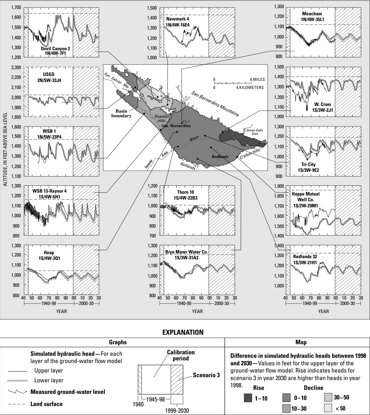
Figure 58. Results from water-management scenario 3 in the San Bernardino area, California, 1999–2030.
