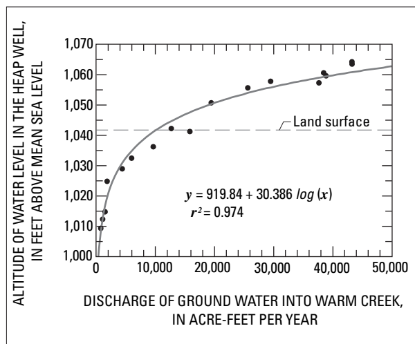
Figure 21. Relation between discharge in Warm Creek and ground-water level in the San Bernardino area, California. Measured discharge data for water years 1943–59 from California Department of Water Resources (1971, table 22, column 1, p. 150). Measured water levels for the Heap well (1S/4W-3Q1) from the USGS.
