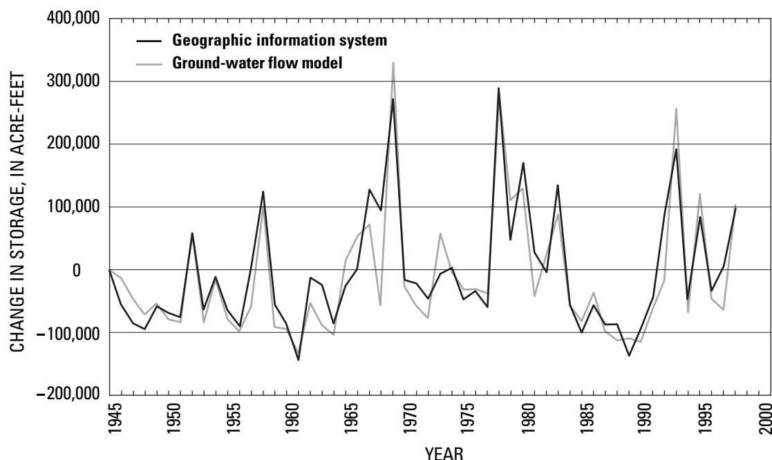
Figure 45. Estimated change in ground-water storage in the San Bernardino area, California, 1945–98. Methods of calculating values with a geographic information system and with the ground-water flow model are described on pages 52–53.
