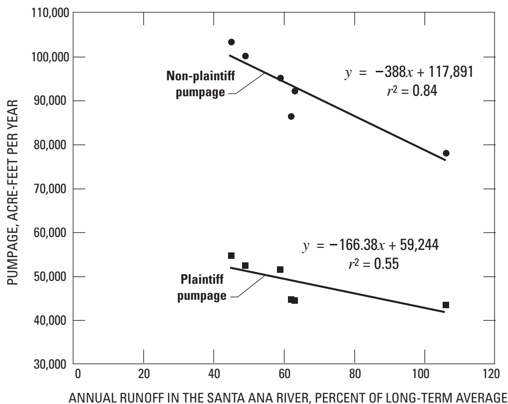
Figure 32. Regression equations used to estimate pumpage in the San Bernardino area, California, 1945–46. All data for 1947–52; refer tables 2 and 10. Runoff data for U.S. Geological Survey gaging station 11051501; long-term average runoff for 1945–98. Plaintiff and non-plaintiff (filed) pumpage data from the Western–San Bernardino Watermaster.
