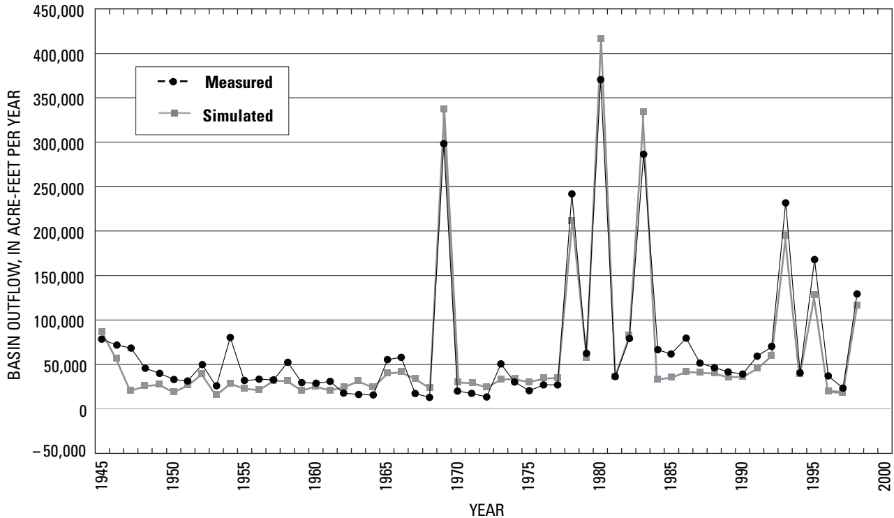
Figure 44. Comparison between measured and simulated surface-water outflow from the San Bernardino area, California, 1945–98.
