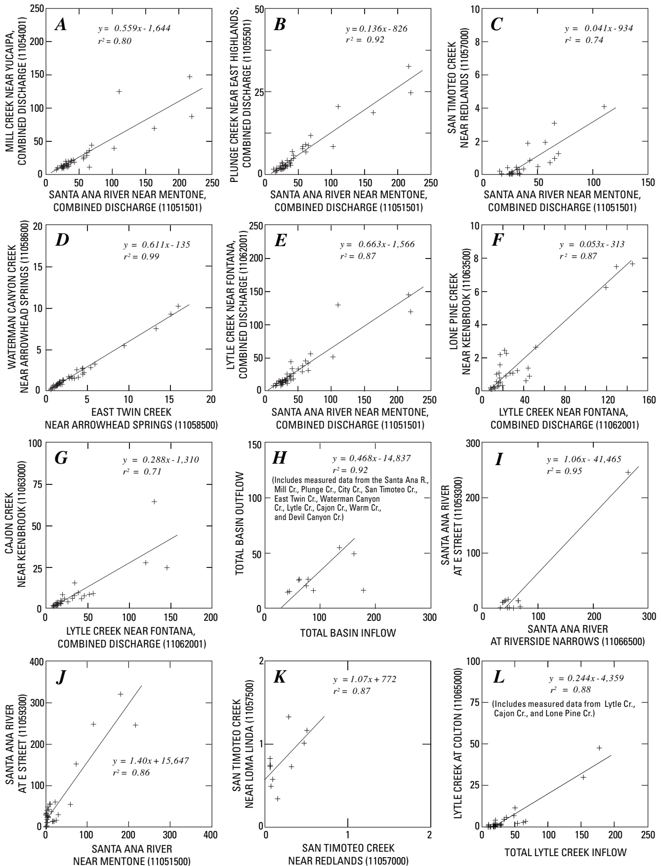
Figure 13. Linear-regression relations used to estimate annual stream discharge in the San Bernardino area, California. Annual data points are shown; values are in thousands of acre-feet per year.
