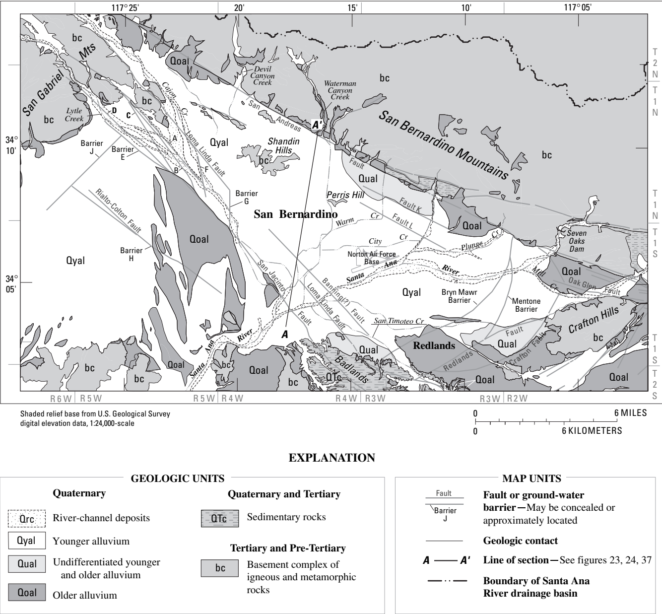
Figure 5. Generalized surficial geology of the San Bernardino area, California, adapted from Morton (1974) and Dutcher and Garrett (1963).
