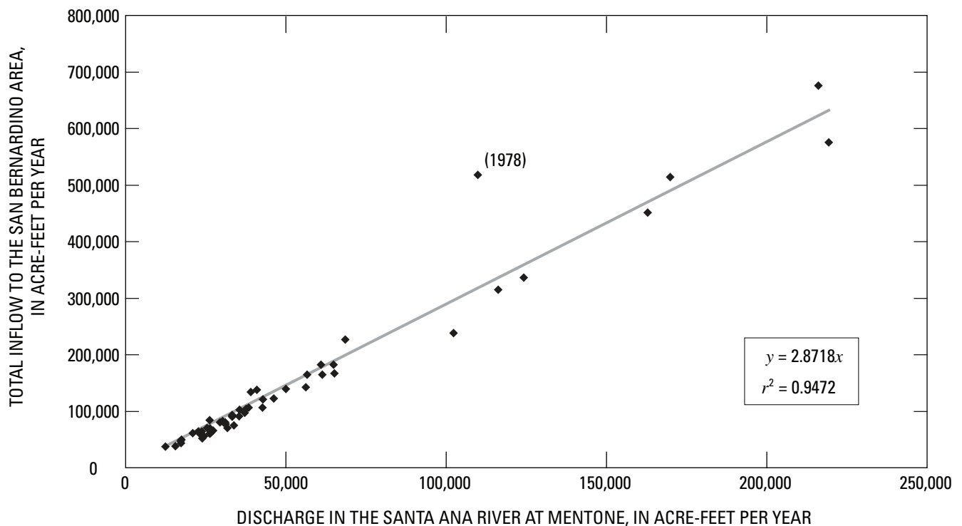
Figure 16. Relation between discharge in the Santa Ana River at the base of the mountains (USGS station 11051501) and total inflow to the San Bernardino area, 1945–98. Values are listed in table 1 . During calendar year 1978, inflow for Lytle and Cajon Creeks was unusually high.
