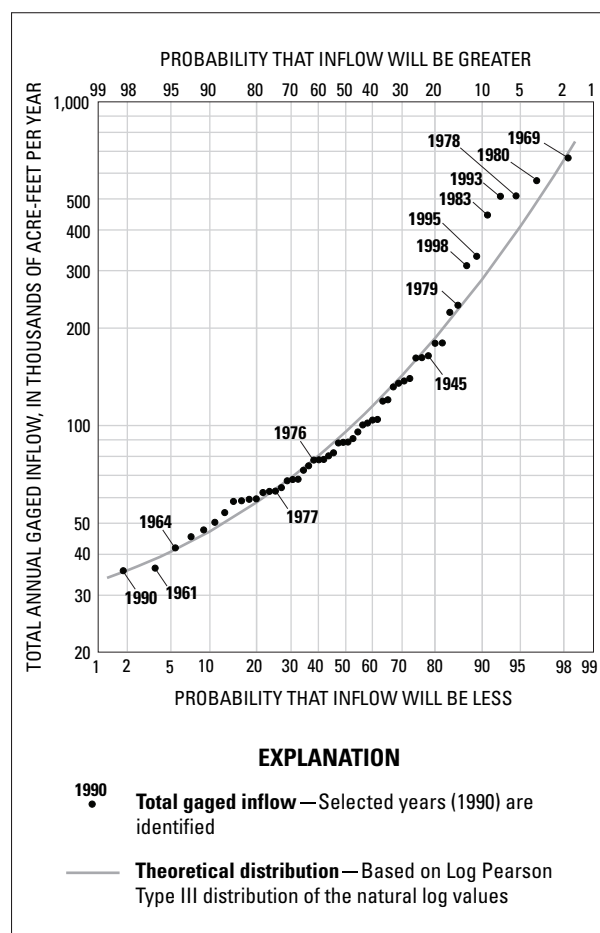
Figure 14. Cumulative probability of annual gaged surface-water inflow for the San Bernardino area, California, 1945–98. Values of inflow are listed in table 1 .
