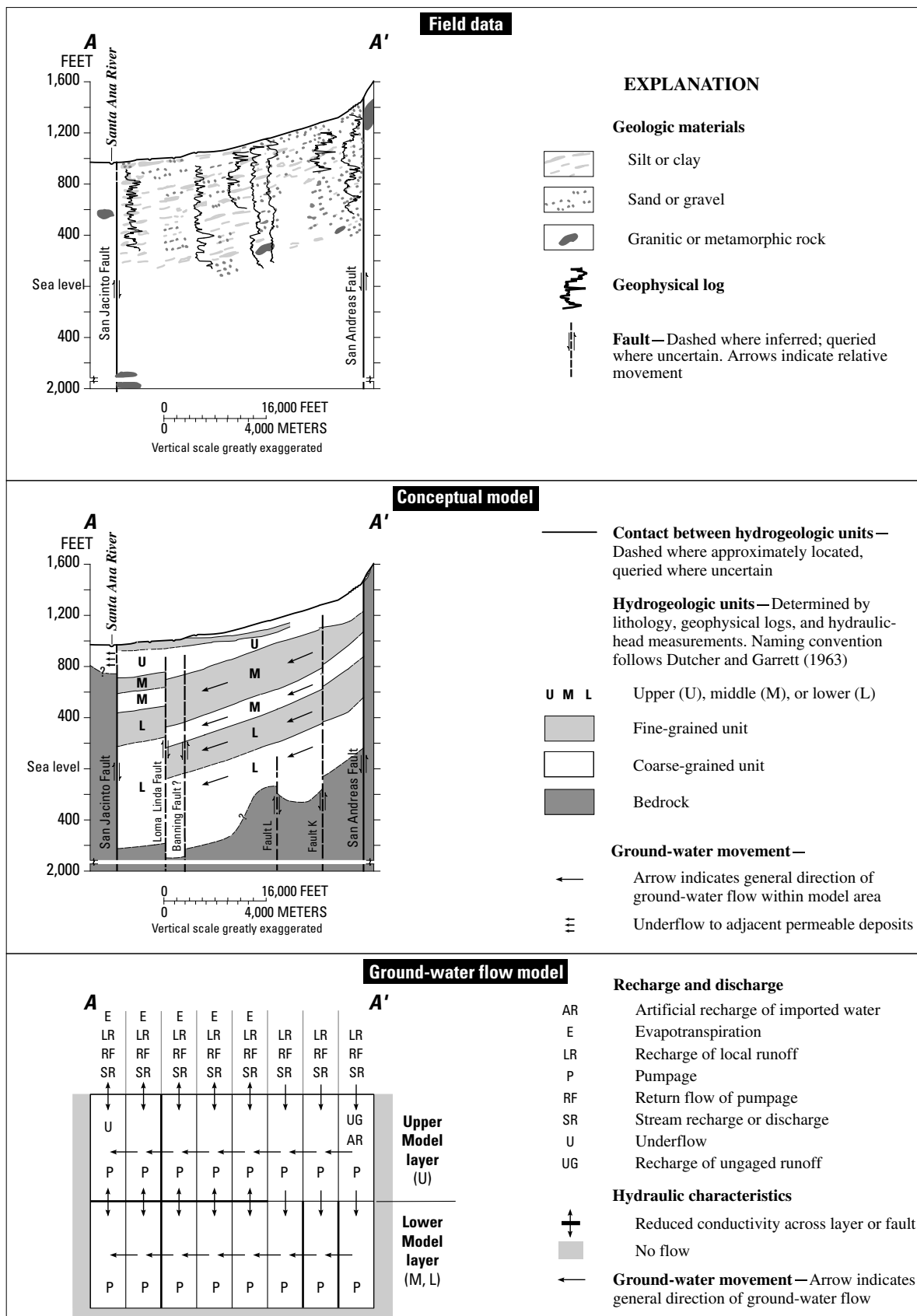
Figure 38. General relations among field data, conceptual model, and ground-water flow model of the San Bernardino area, California.
