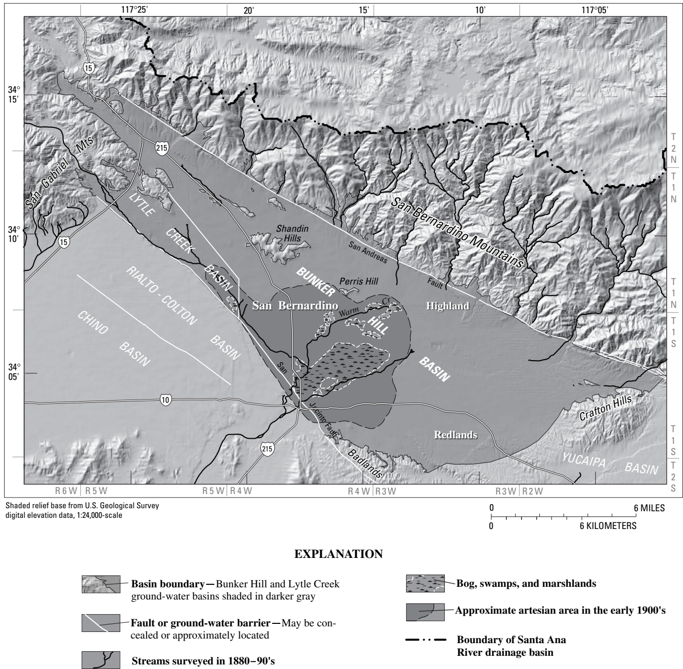
Figure 9. Historical hydrologic conditions in the San Bernardino area, California, circa 1880. Adapted from Hall (1888), Mendenhall (1905), and Fife and others (1974).
