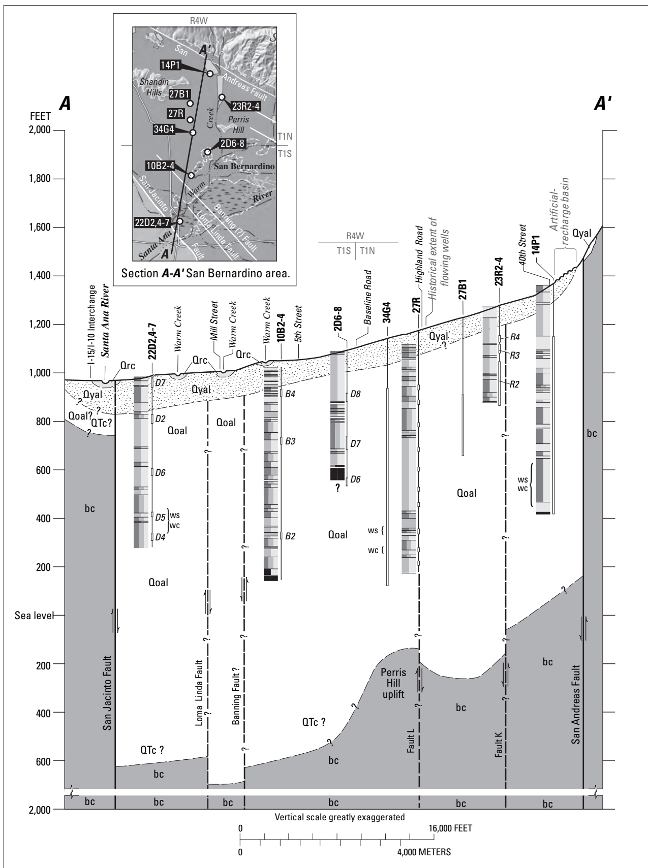
Figure 23. Representative geologic section A-A' and stratigraphic units in the San Bernardino area, California.
