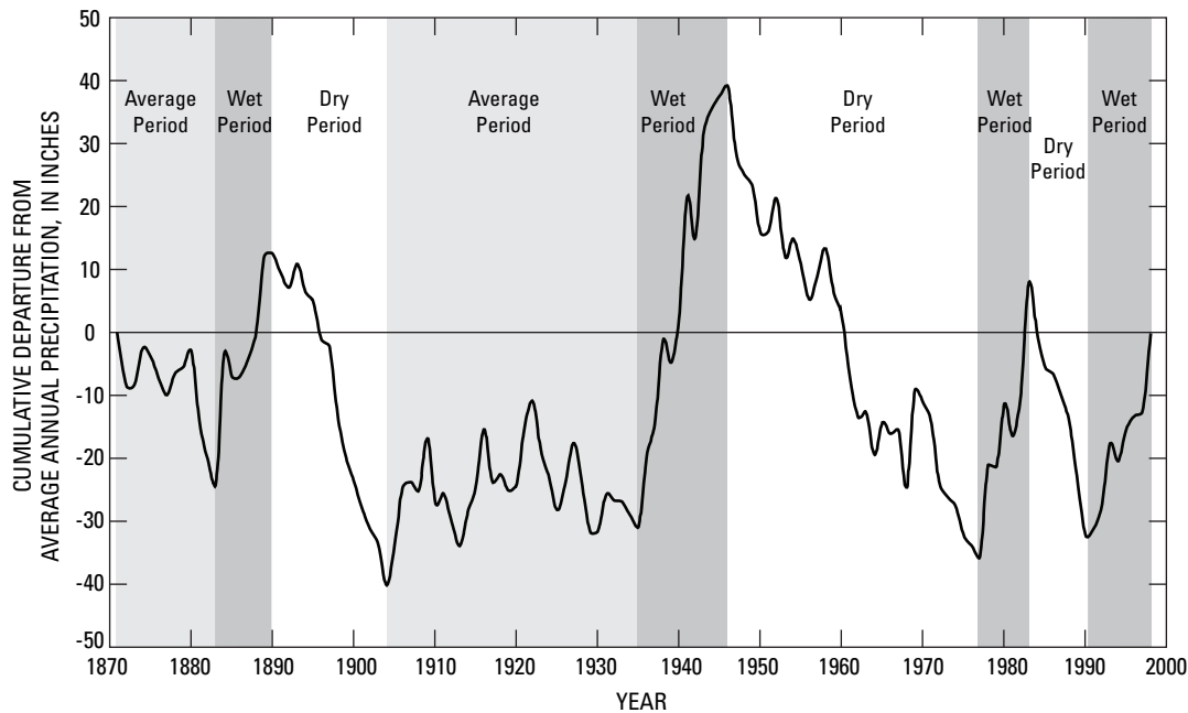
Figure 7. Cumulative departure from average annual precipitation at San Bernardino, California, 1871–1998. Data from the San Bernardino County Flood Control District, station 47723.
