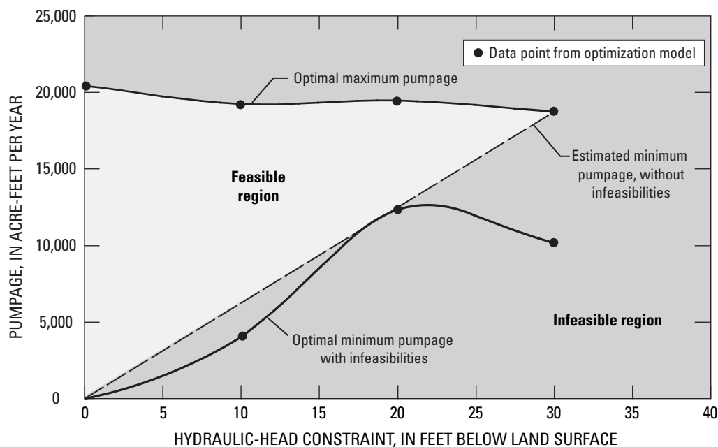
Figure 65. Minimum and maximum pumpage for scenario 6 for the San Bernardino area, California. The apparent decrease in optimal minimum pumpage is caused by omitting infeasible head constraints from the optimization model. The actual minimum pumpage required to lower high ground-water levels, as indicated by the dashed line, is likely to be somewhat greater than that predicted by the optimization model. The maximum pumpage that can be obtained without having ground-water levels fall too low is approximately 20,000 acre-feet per year.
