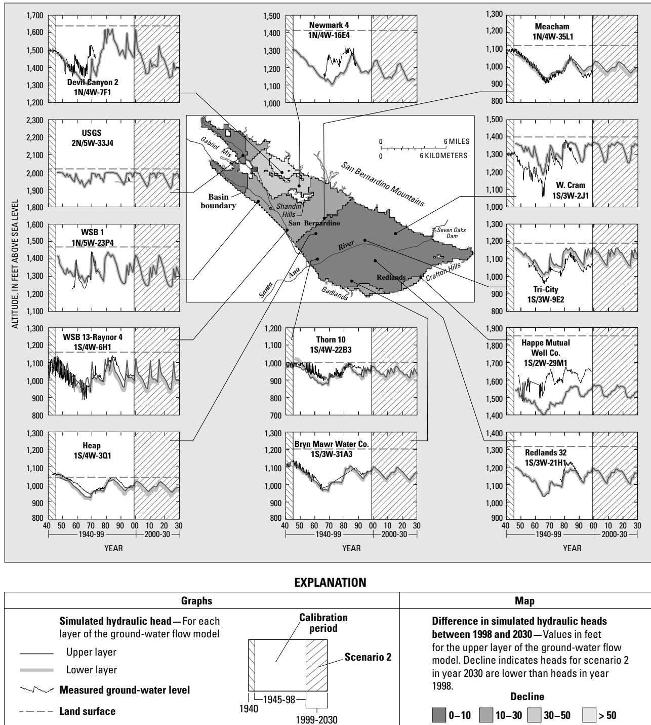
Figure 57. Results from water-management scenario 2 in the San Bernardino area, California, 1999–2030.
