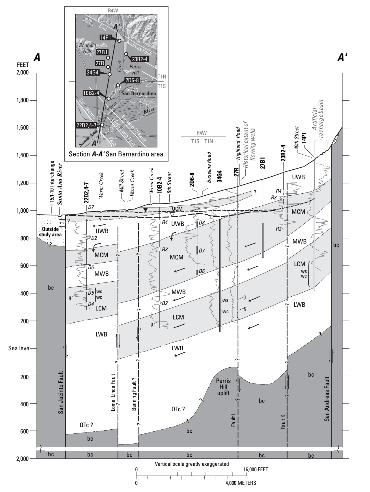
Figure 24. Section A-A' showing major hydrogeologic units, geophysical logs, and direction of ground-water flow in the San Bernardino area, California.
