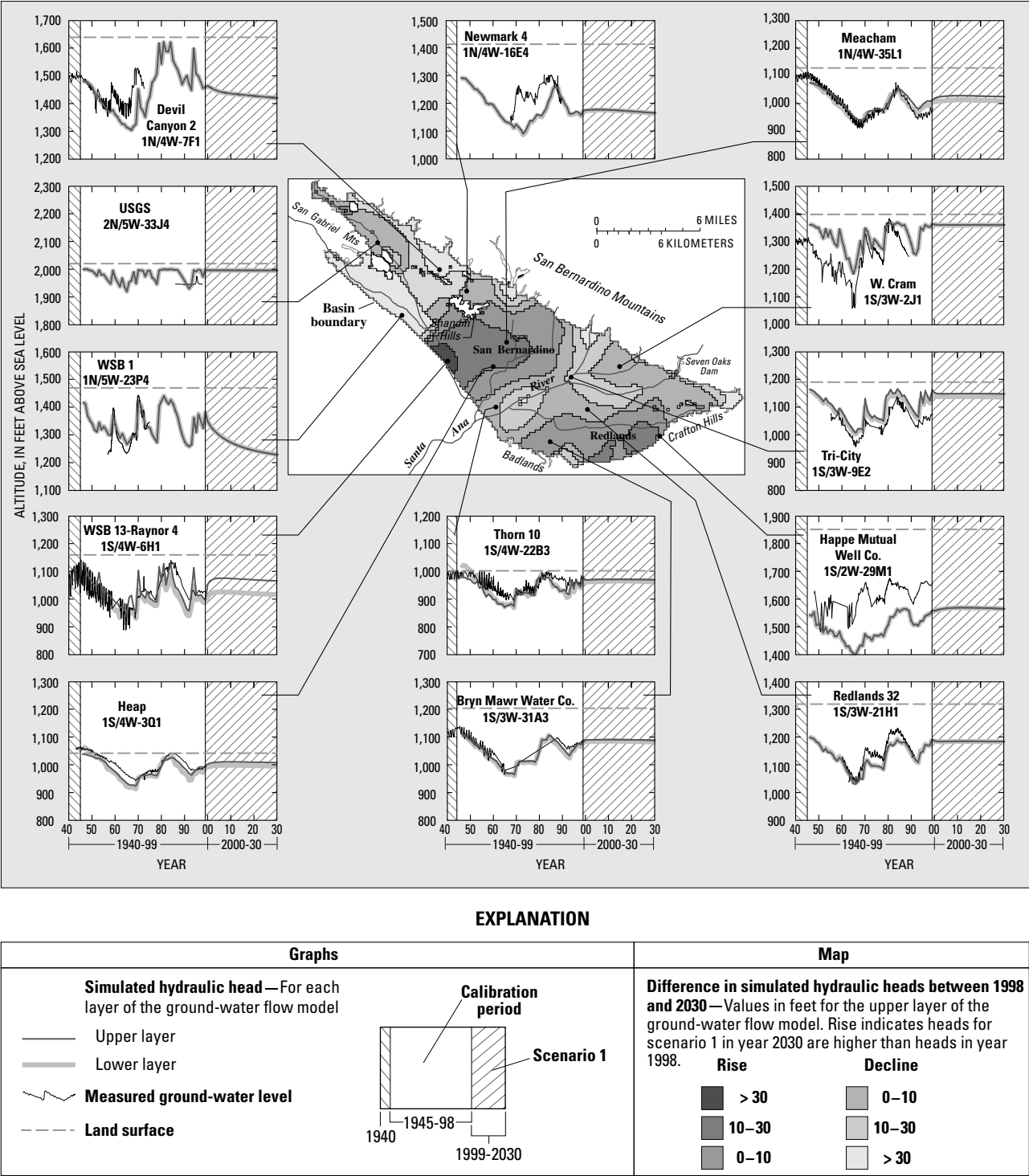
Figure 56. Results from water-management scenario 1 in the San Bernardino area, California, 1999–2030.
