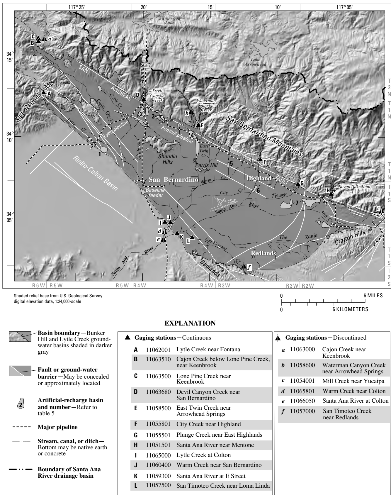
Figure 11. General features of the surface-water system in the San Bernardino area, California, 1998.
