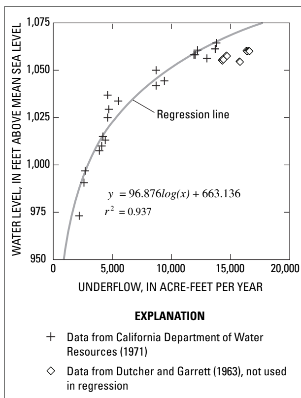
Figure 28. Relation between water level in the Heap well (1S/4W-3Q1) and underflow across the San Jacinto fault near the Santa Ana River.
