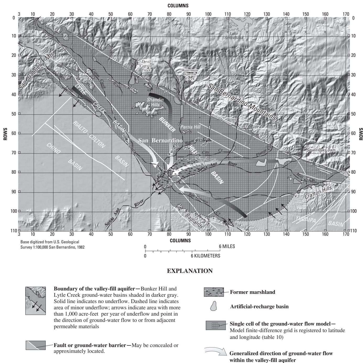
Figure 39. Location, orientation, and boundary conditions of the ground-water flow model of the San Bernardino area, California.
