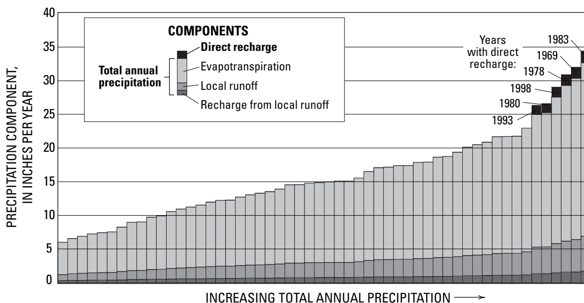
Figure 18. Components of precipitation on the Bunker Hill and Lytle Creek basins in the San Bernardino area, California, 1945–98. Precipitation measured at San Bernardino County Flood Control District station 47723. Selected years are identified.
