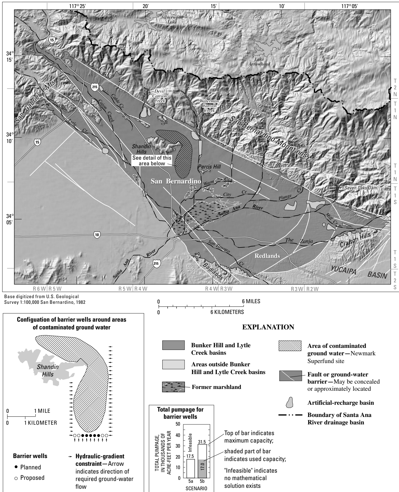
Figure 61. Results from water-management scenario 5 in the San Bernardino area, California, 1999–2030. Scenario 5a uses the 5 planned wells; scenario 5b uses the 5 planned and 4 proposed wells. Scenario 5a uses all hydraulic-gradient constraints; scenario 5b uses only the 9 hydraulic-gradient constraints along the southern boundary.
