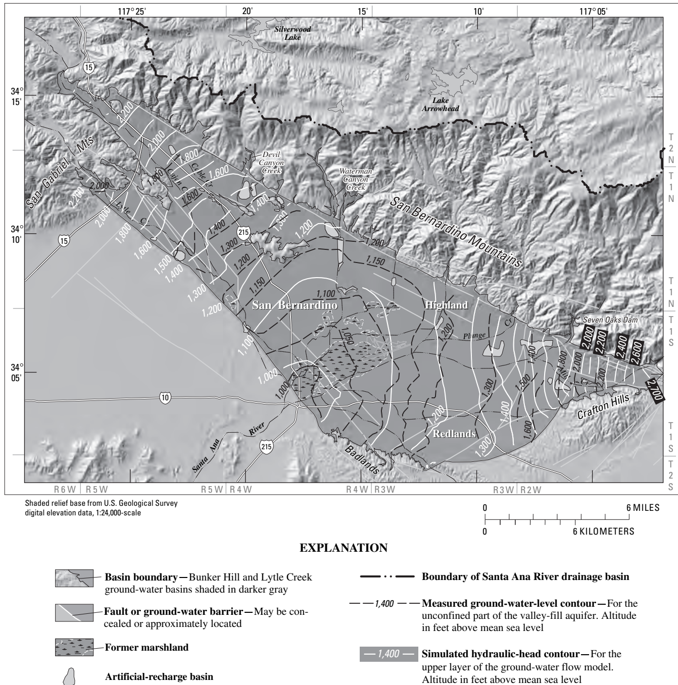
Figure 42. Measured ground-water levels and simulated hydraulic heads for the unconfined part of the valley-fill aquifer in the San Bernardino area, California, 1945. Measured contours adapted from unpublished map by F.B. Laverty (San Bernardino Valley Municipal Water District, written commun., 1998).
