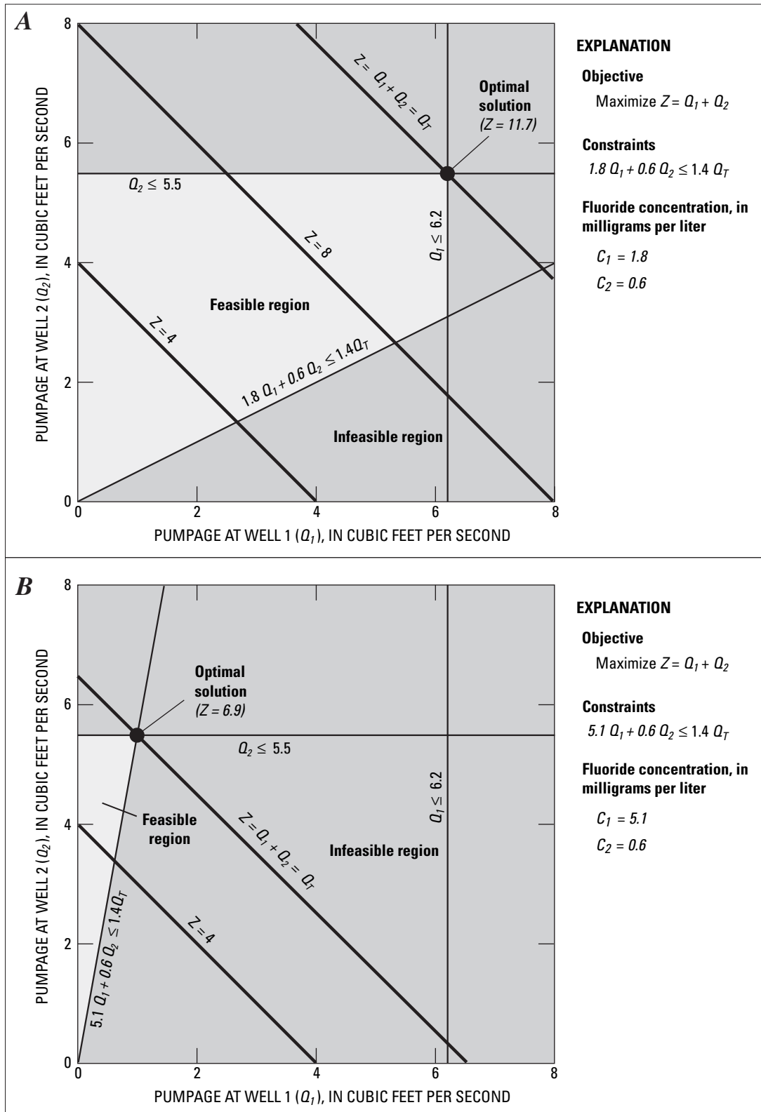
Figure 46. Graphical solution of a simple constrained optimization model. Graphs A and B show optimal solutions for fluoride concentrations in well 1 of 1.8 and 5.1 milligrams per liter, respectively.
